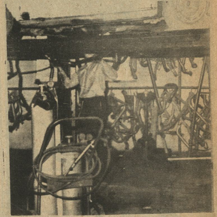
ROGERS also has a complete exhaust system service and can build exhaust systems to the customer's specifications. David Bethune, full-time mechanic, is shown as he installs an exhaust pipe. One of the services available at Rogers is custom dual exhaust systems.
