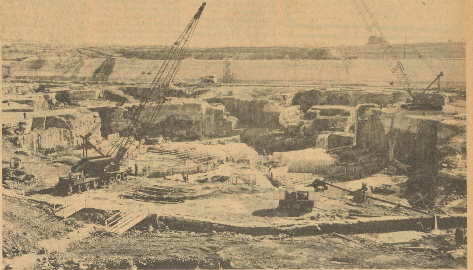
Overall View Of Unit One Reactor Building--Looking South
