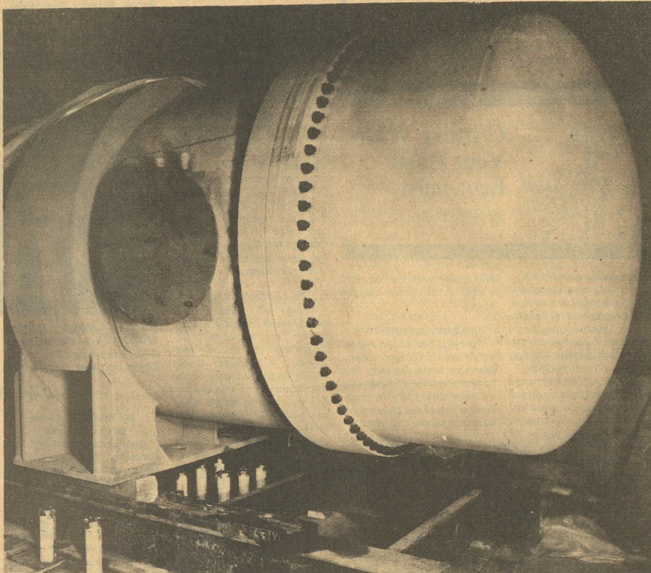
Component cooling heat exchanger for elevation 452.0 in unit 1 reactor auxiliary area, looking north.
